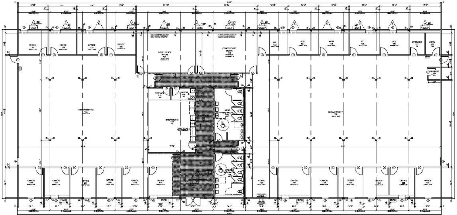
1 FLOOR PLAN 1/8"=1'-0" SQUARE FOOTAGE - 13104 S.F. OCCUPANCY LOAD - 75
